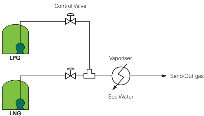
Figure 7.14 – LNG/LPG Enrichment.
