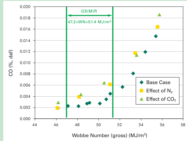
Figure 2.7 – Effect of Natural Gas 'Dilution' with Nitrogen and Carbon Dioxide
