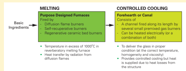
Figure 6.12 – Basic Process of Glass Manufacturing.
