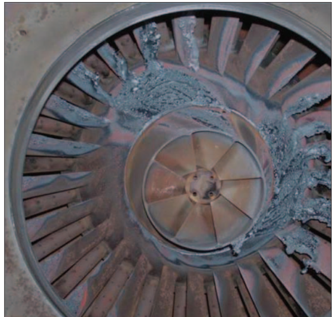
Figure 1.1 – Gas turbine – Damage from Flashback. (Reproduced with permission of E.ON)
