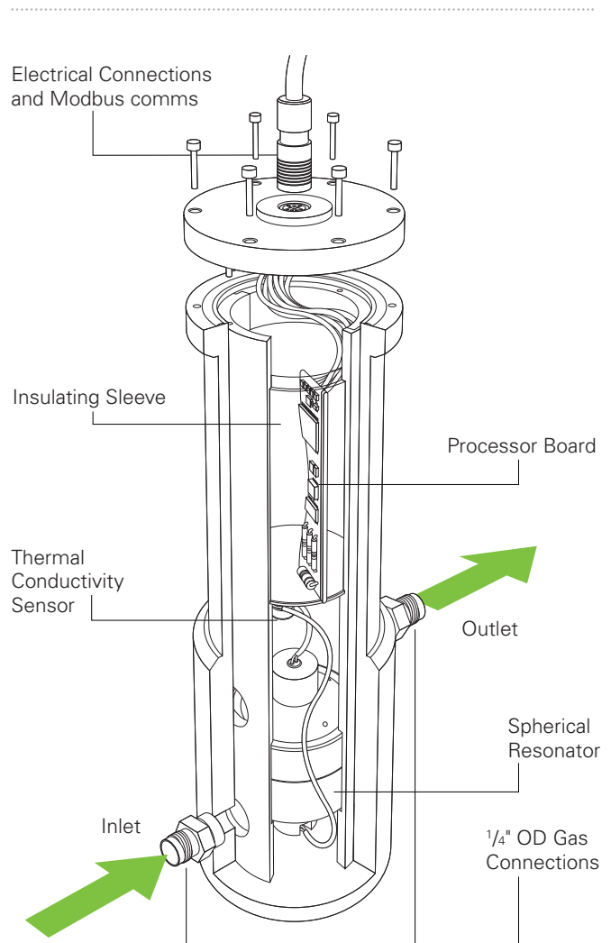
Figure 7.20 – The GasPT™
