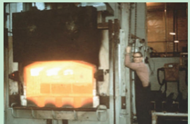
Figure 2.8 – Gas-fired steel reheat furnace.
