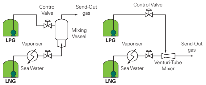
Figure 7.13 – Gas/LPG Enrichment Methods.
