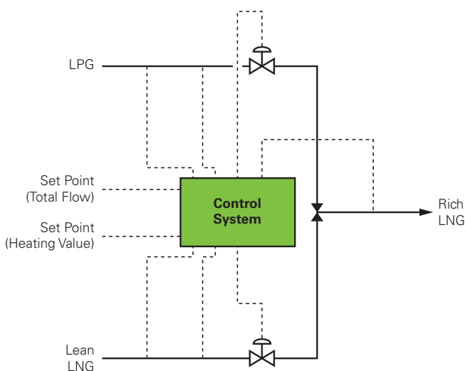
Figure 7.18 – Simplified Control Scheme for LNG Enrichment with LPG.
