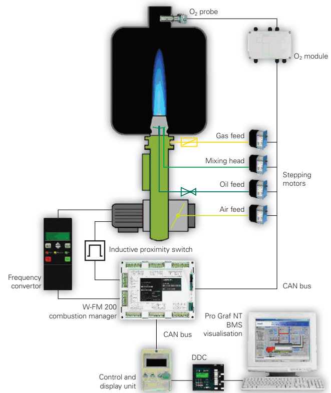
Figure 7.22 – An Oxygen Trim Set-up.
