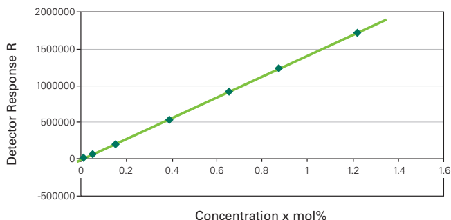
Figure 3.2 – Iso-butane: Equation of Detector Response. R = 1391922 * x
