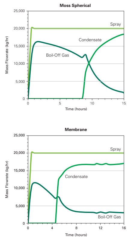
Figure 4.19 – Cooldown Rate for Moss and Membrane Carriers.
