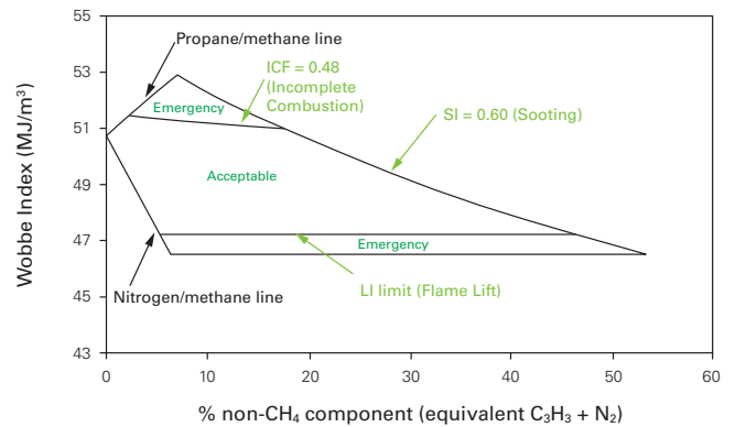
Figure 2.4 – Dutton Diagram with GS(M)R Limits.
