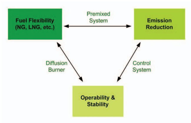
Figure 6.3 – Relationship between Fuel Flexibility, Combustor Type and Emissions.
