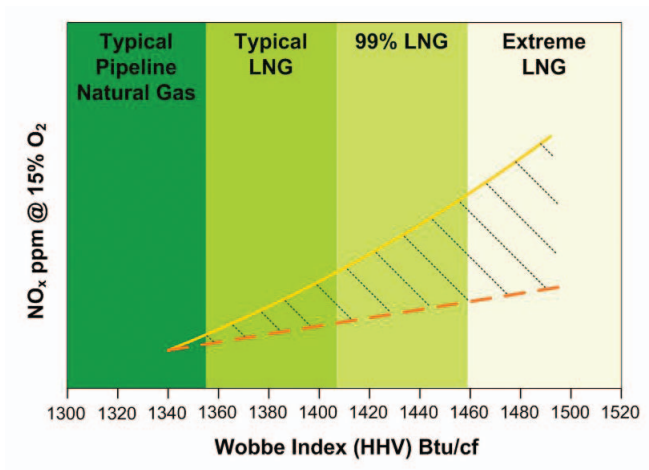
Figure 6.4 – NO x Emissions and Wobbe Index.
