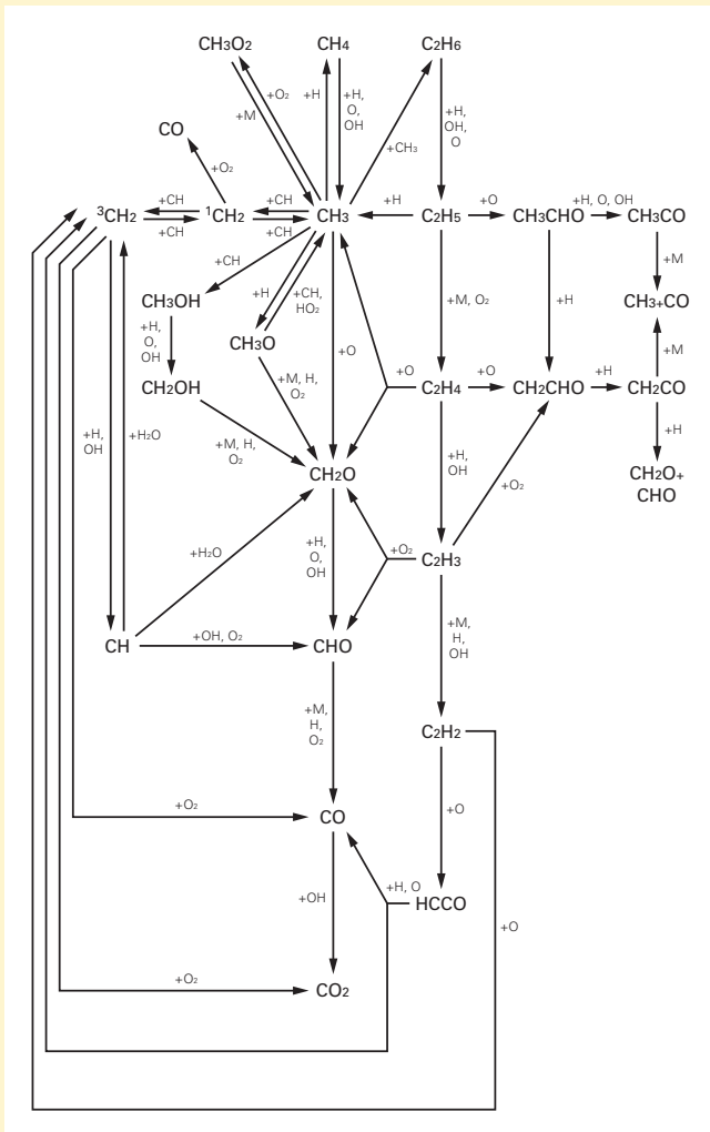
Figure 2.1 – The Complexity of Methane Oxidation. (Source: www.ivr.uni-heidelberg.de/groups/readflow )
