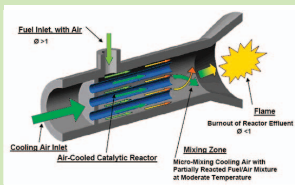
Figure 6.7 – Catalytic Combustor. (Reproduced with permission of Combustion Inc)
