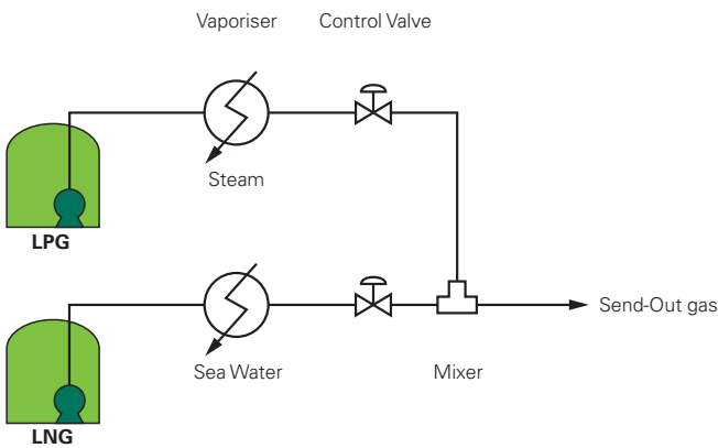
Figure 7.12 – Gas/Gas Enrichment.
