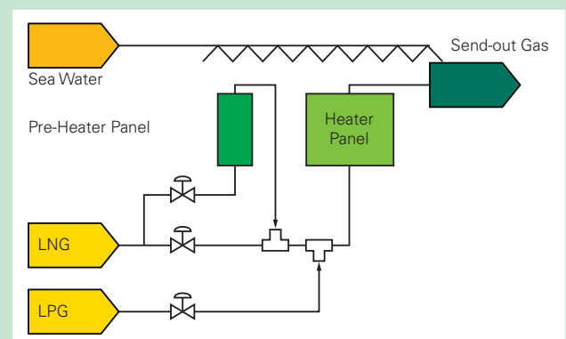
Figure 7.15 – Outline of ORV with LNG/LPG Enrichment.
