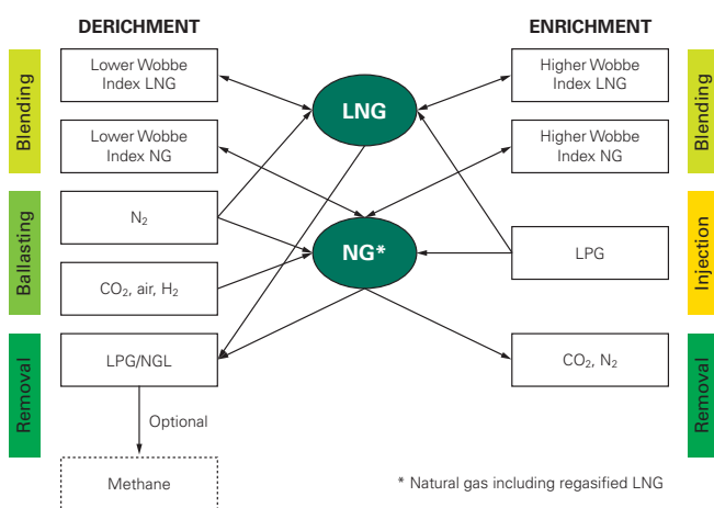
Figure 7.2 – Summary of Quality Management Techniques for LNG and Natural Gas.
