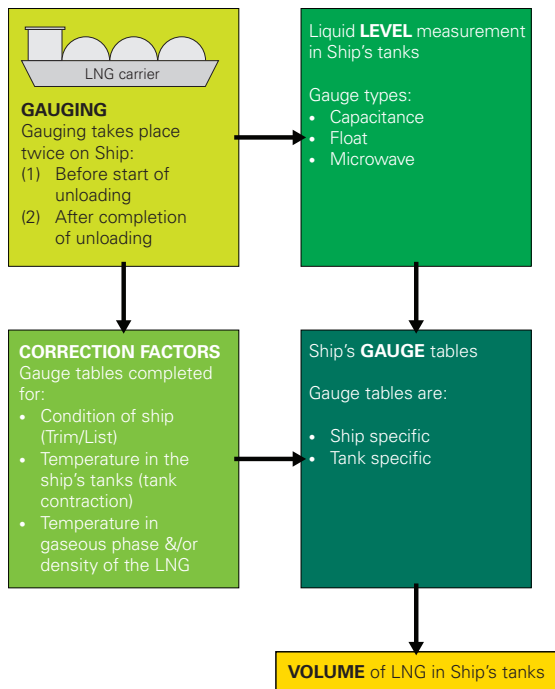
Figure 4.17 – Gauging Process.
